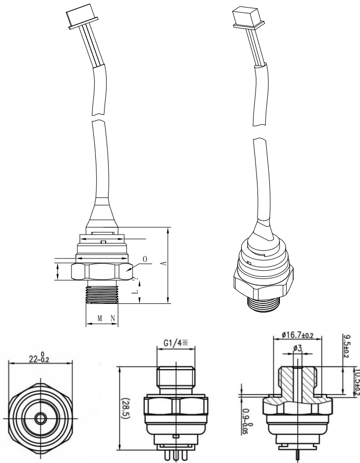
Dimension in:mm
