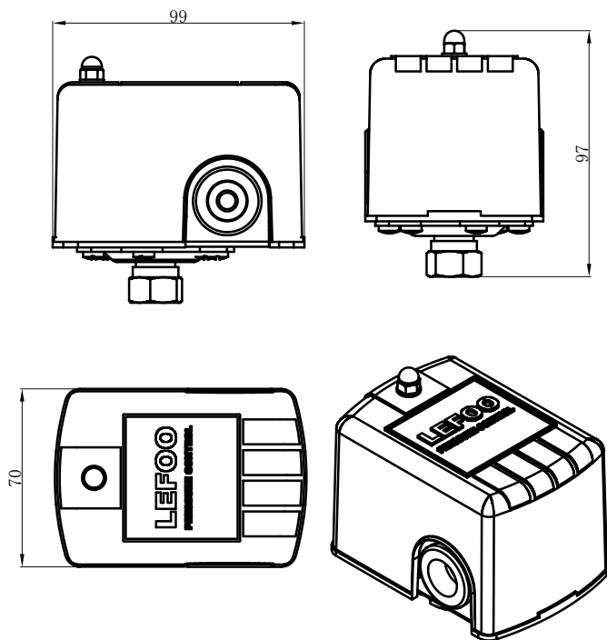
Dimension in:mm
