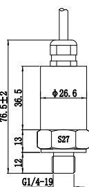
Current-voltage type M12 cable outlet
