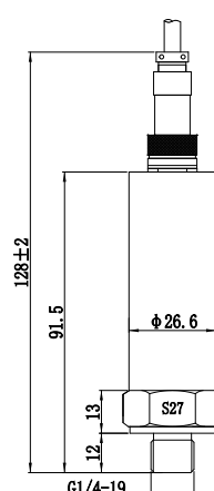
RS485 Gx12 aviation connector
