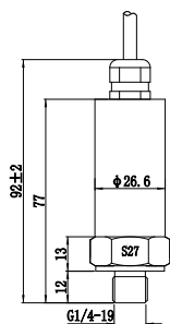
RS485 M12 cable outlet
